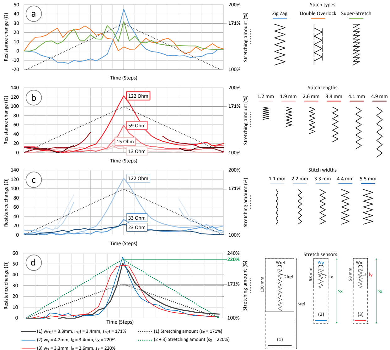
Figure 4: Resulting changes in resistance ( \Omega ) for varying (a) stitch types, (b) stitch lengths (fixed stitch width = 3.3 mm), (c) stitch widths (fixed stitch length = 3.4 mm), and (d) stretch sensor samples with different elasticities, stitch widths and stitch lengths.
