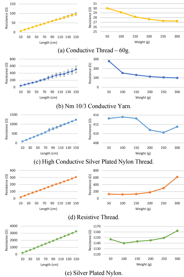
Figure 2: Changes in resistance (Ω) over different yarn lengths (left) and over different amounts of applied tension (right).
