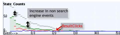
Figure 5: The State Counts Panel is a bar chart with event ordinality on the x-axis and event counts on the y-axis for all events (gray bars) and individual event states (stacked and color-coded). Here, the later events were predominantly non-search engine events, as indicated by the increasingly large gap between the total event counts and coded event state counts.
