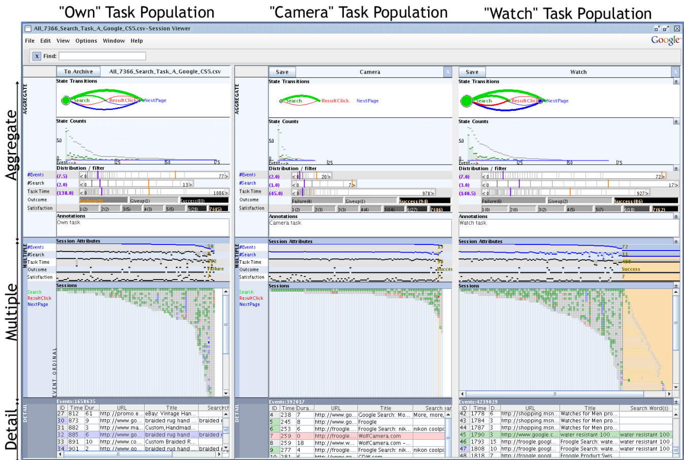
Figure 3: The main screen of Session Viewer showing user study data. Session Viewer displays multiple session populations in vertical views. From left to right: the "Own" Task population where participants performed their own self-created tasks; the Camera Task population with searches for a camera feature given the brand and model; and the Watch Task population with searches to locate a watch based on given criteria. For each population, the session logs are shown in the Aggregate, the Multiple, and the Detail Panes.
